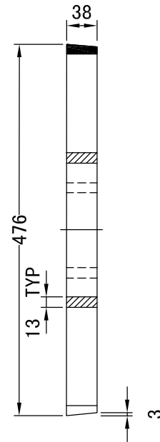
SECTION C-C
