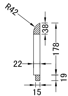
SECTION E-E
