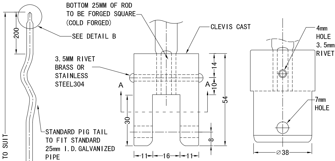
DETAIL A
