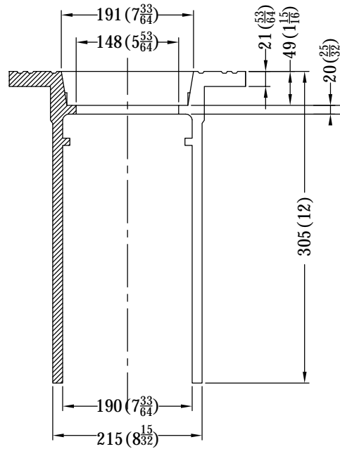
SECTION A-A VALVE BOX
