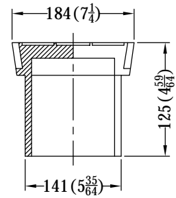
SECTION B-B VALVE BOX
